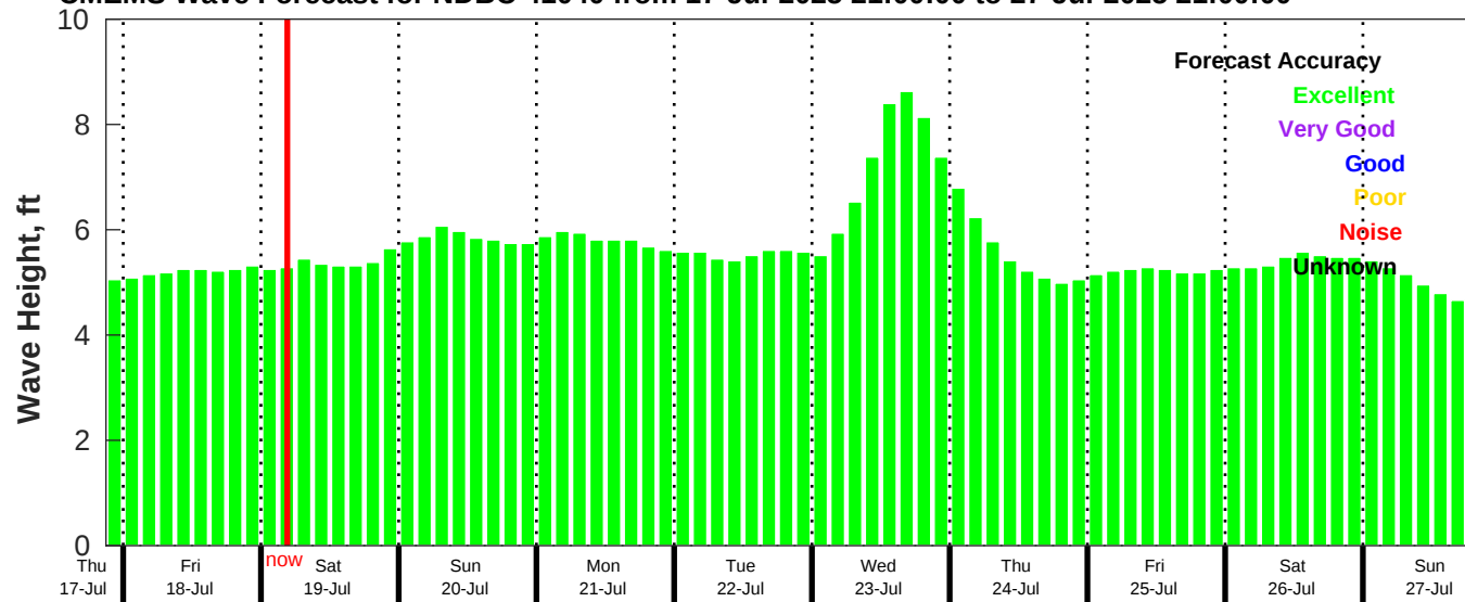
CMEMS Wave Forecast for NDBC 41040 from 17-Jul-2025 21:00:00 to 27-Jul-2025 21:00:00
