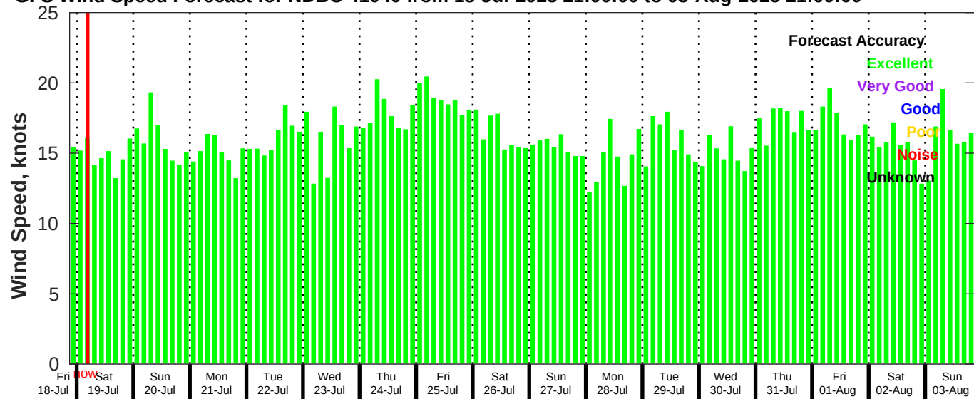
GFS Wind Speed Forecast for NDBC 41040 from 18-Jul-2025 21:00:00 to 03-Aug-2025 21:00:00
