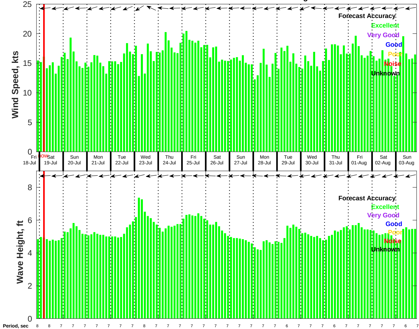
Wind & Wave Forecast for NDBC 41040 from 18-Jul-2025 21:00:00 to 03-Aug-2025 21:00:00
