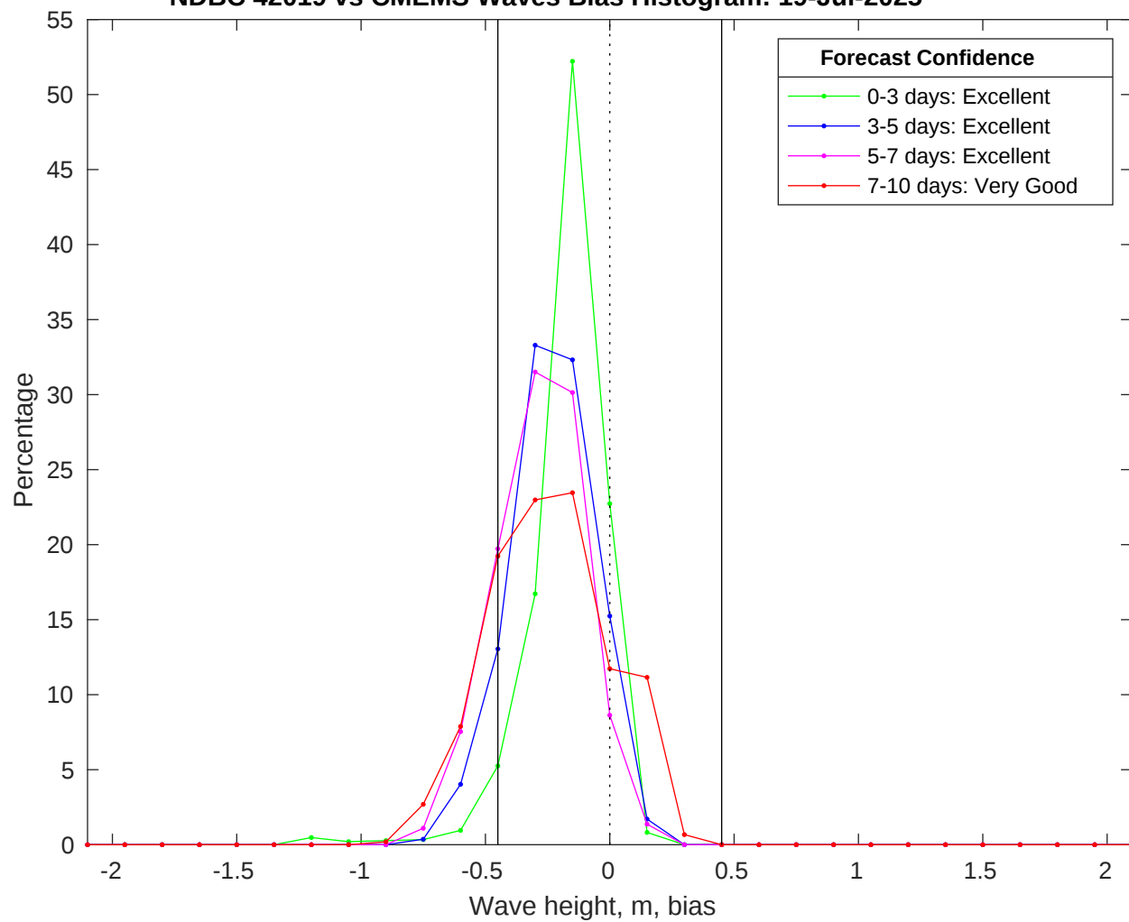
NDBC 42019 vs CMEMS Waves Bias Histogram: 19-Jul-2025
