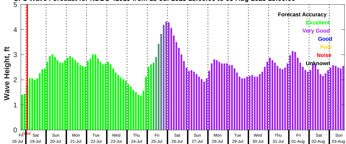
GFS Wave Forecast for NDBC 42019 from 18-Jul-2025 18:00:00 to 03-Aug-2025 18:00:00
