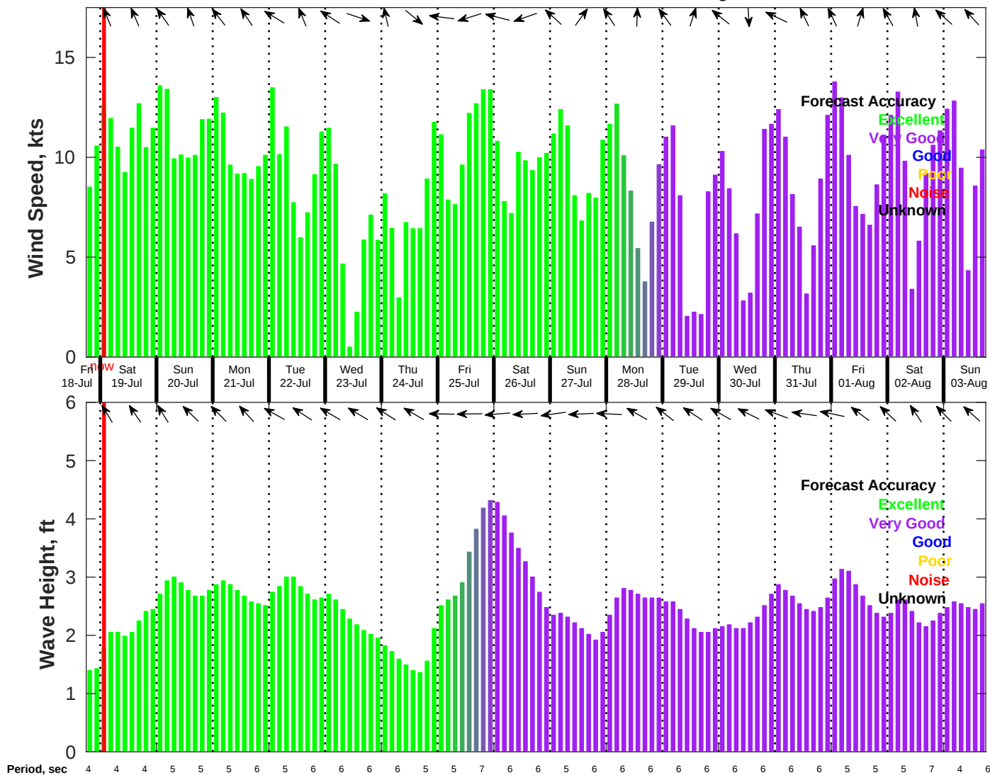
Wind & Wave Forecast for NDBC 42019 from 18-Jul-2025 18:00:00 to 03-Aug-2025 18:00:00
