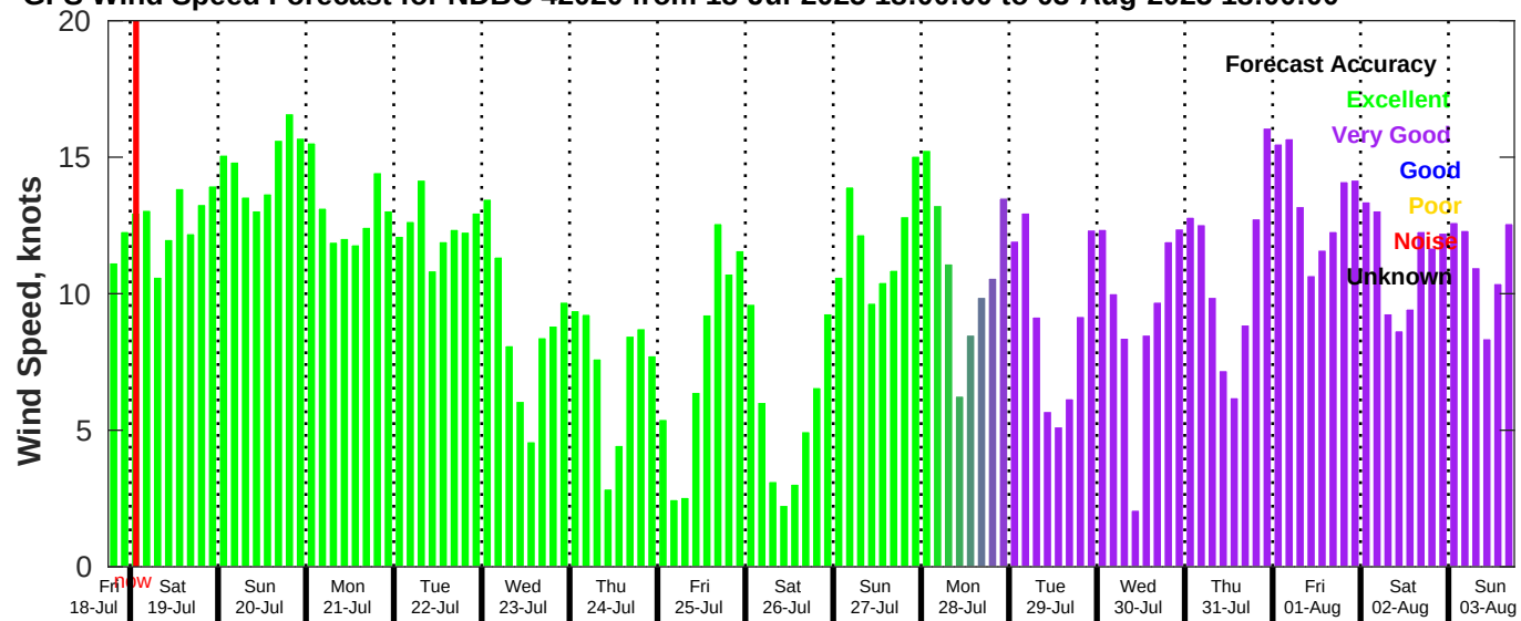
GFS Wind Speed Forecast for NDBC 42020 from 18-Jul-2025 18:00:00 to 03-Aug-2025 18:00:00
