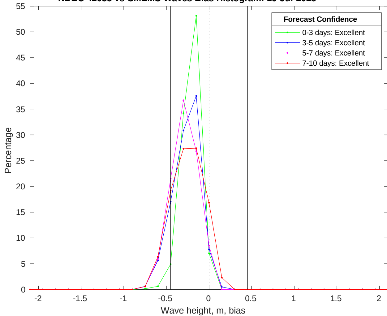
NDBC 42035 vs CMEMS Waves Bias Histogram: 19-Jul-2025
