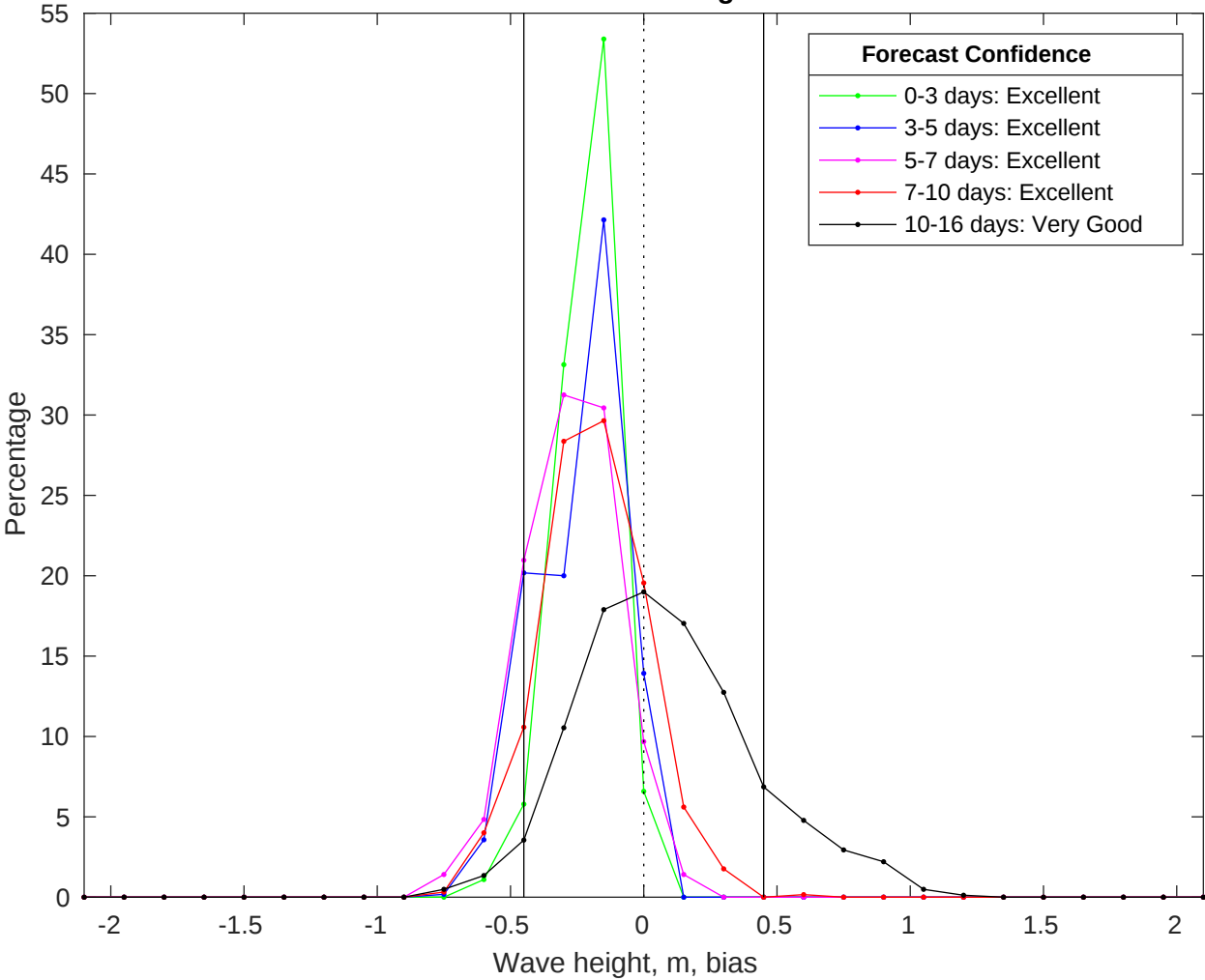
NDBC 42035 vs GFS Waves Bias Histogram: 19-Jul-2025
