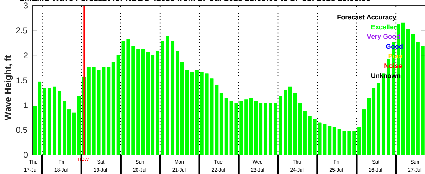
CMEMS Wave Forecast for NDBC 42035 from 17-Jul-2025 18:00:00 to 27-Jul-2025 18:00:00
