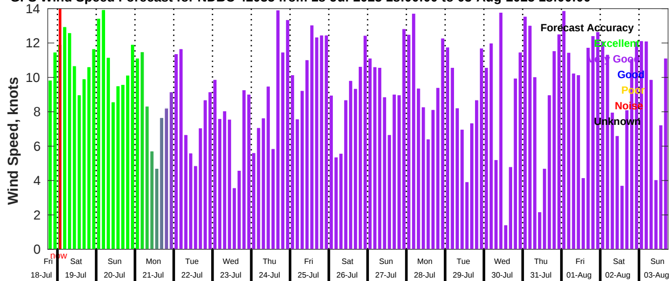
GFS Wind Speed Forecast for NDBC 42035 from 18-Jul-2025 18:00:00 to 03-Aug-2025 18:00:00
