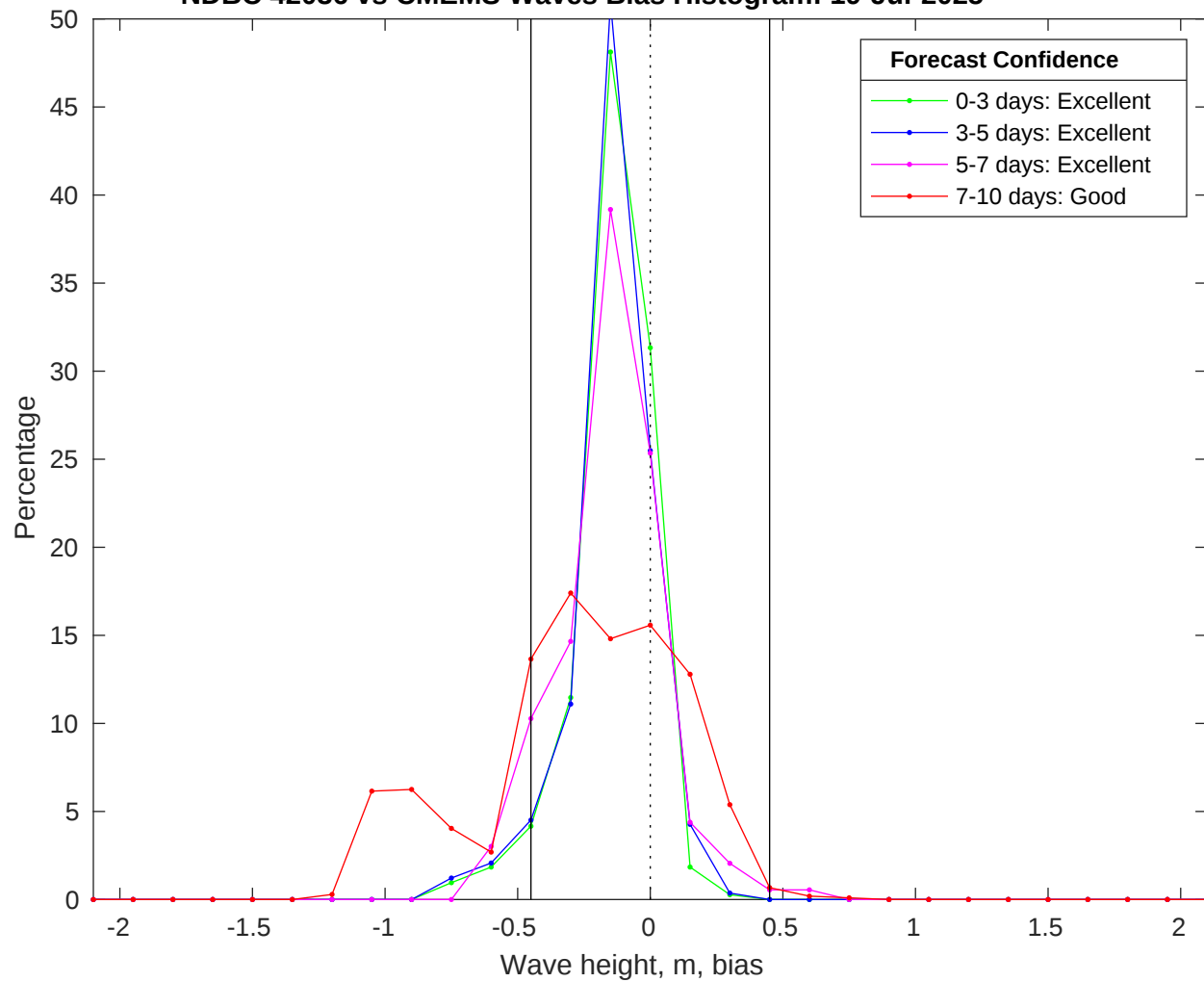
NDBC 42036 vs CMEMS Waves Bias Histogram: 19-Jul-2025
