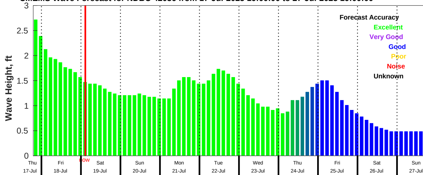
CMEMS Wave Forecast for NDBC 42036 from 17-Jul-2025 19:00:00 to 27-Jul-2025 19:00:00
