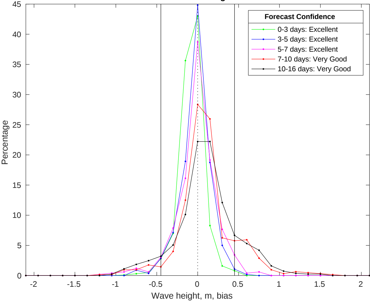
NDBC 42040 vs GFS Waves Bias Histogram: 19-Jul-2025
