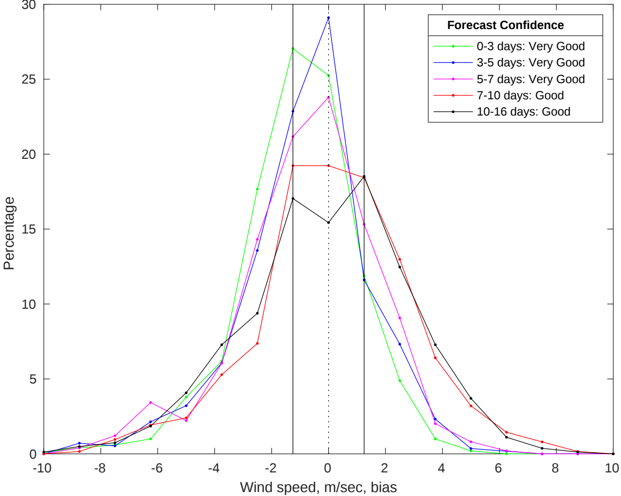
NDBC 42040 vs GFS Winds Bias Histogram: 19-Jul-2025
