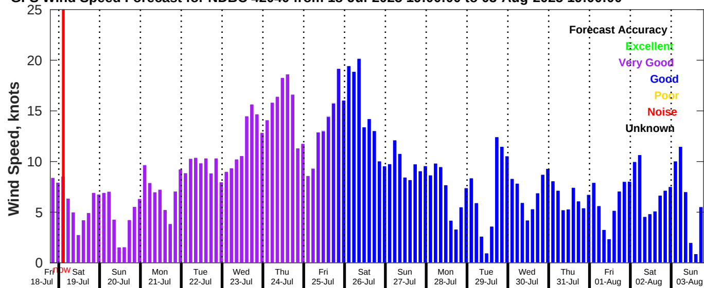
GFS Wind Speed Forecast for NDBC 42040 from 18-Jul-2025 19:00:00 to 03-Aug-2025 19:00:00
