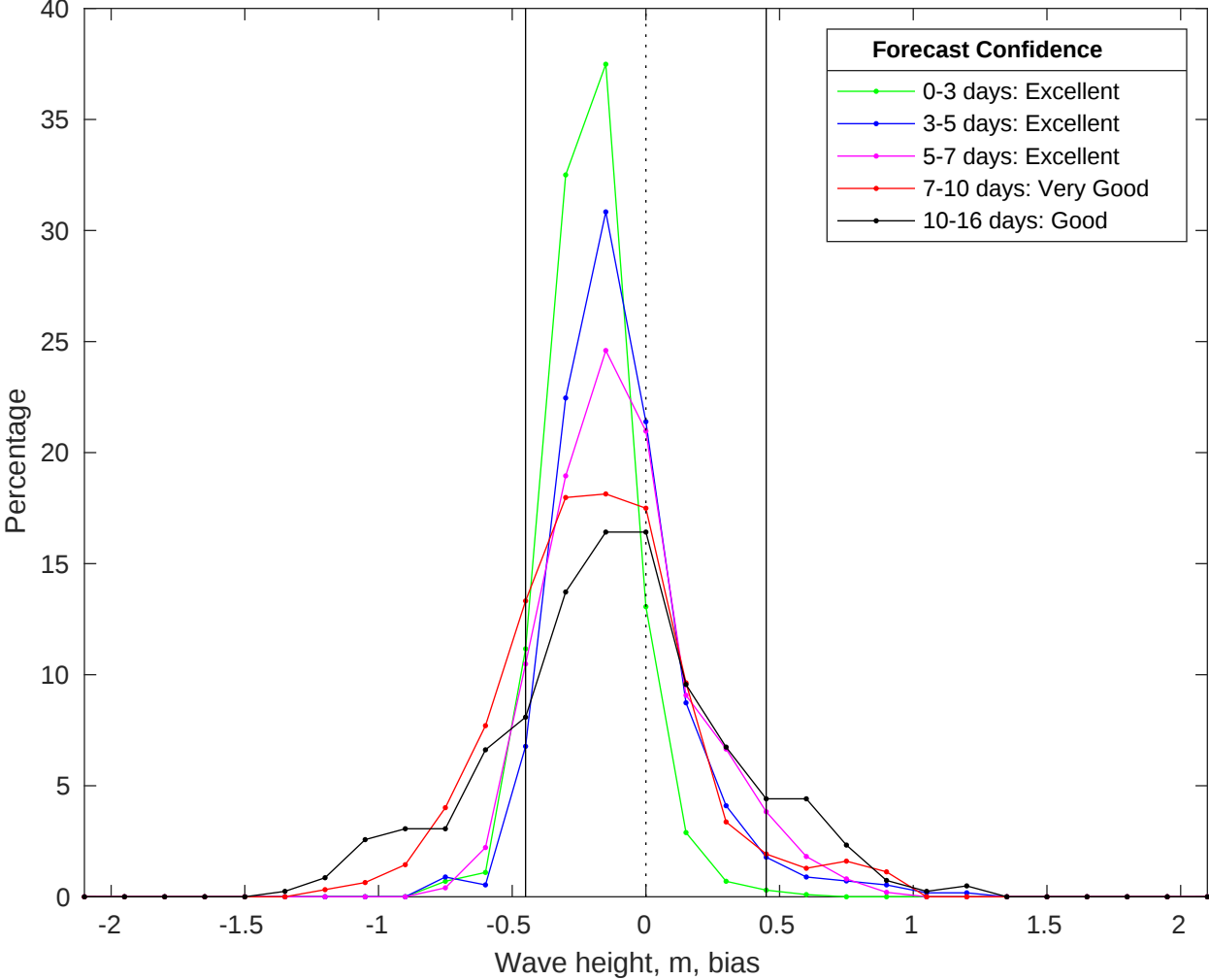
NDBC 46011 vs GFS Waves Bias Histogram: 19-Jul-2025
