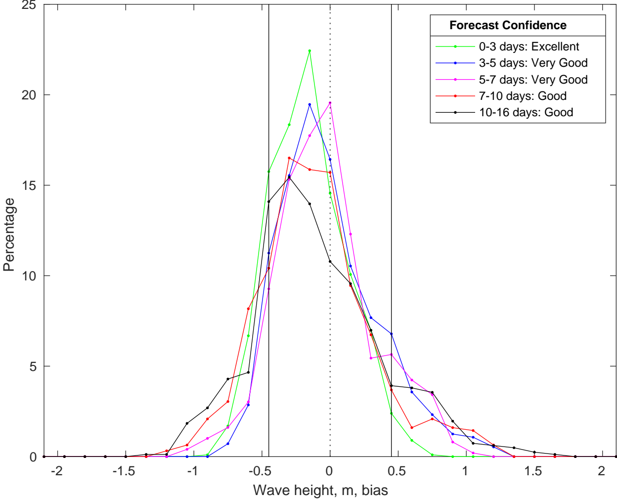
NDBC 46028 vs GFS Waves Bias Histogram: 19-Jul-2025
