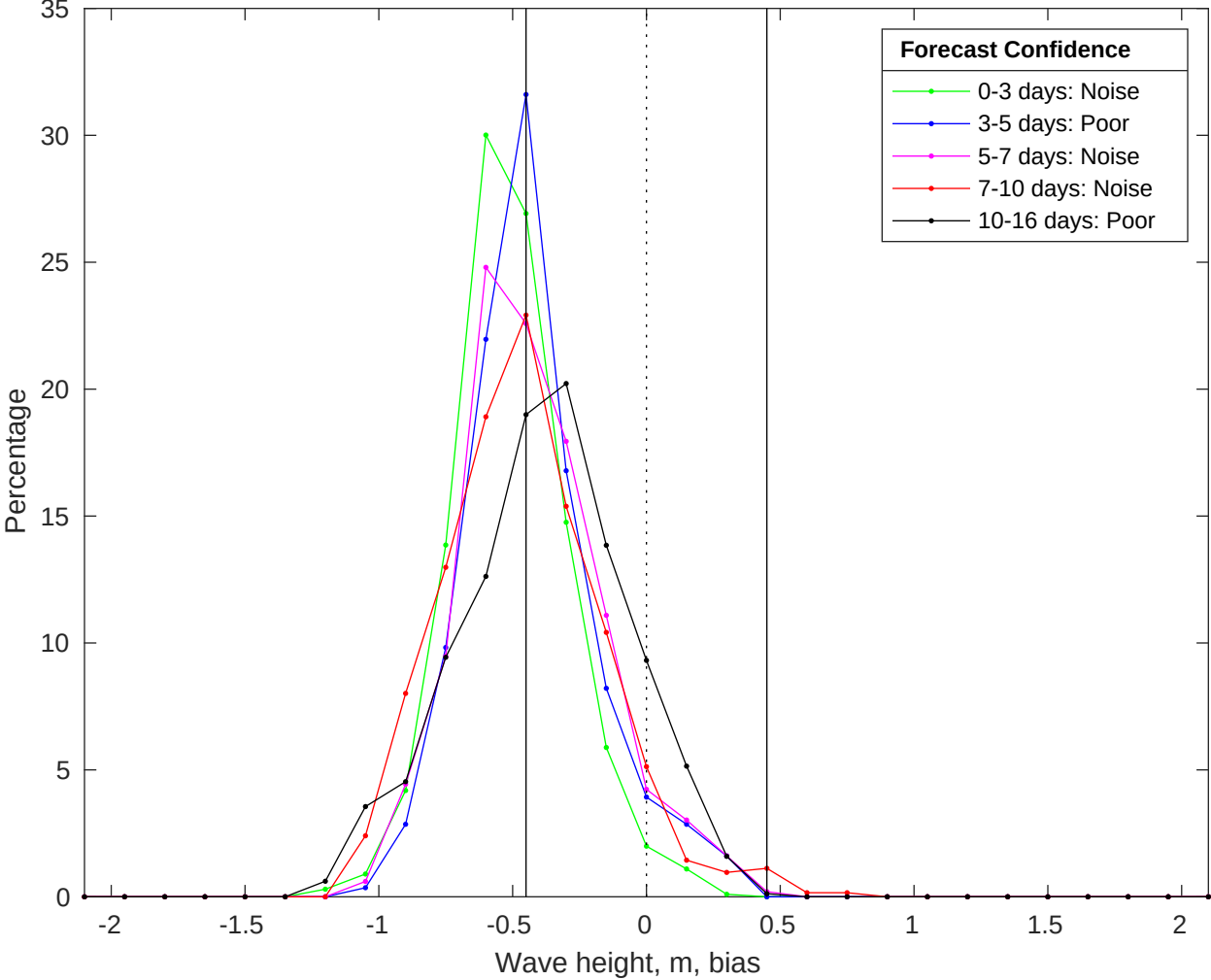
NDBC 46054 vs GFS Waves Bias Histogram: 19-Jul-2025
