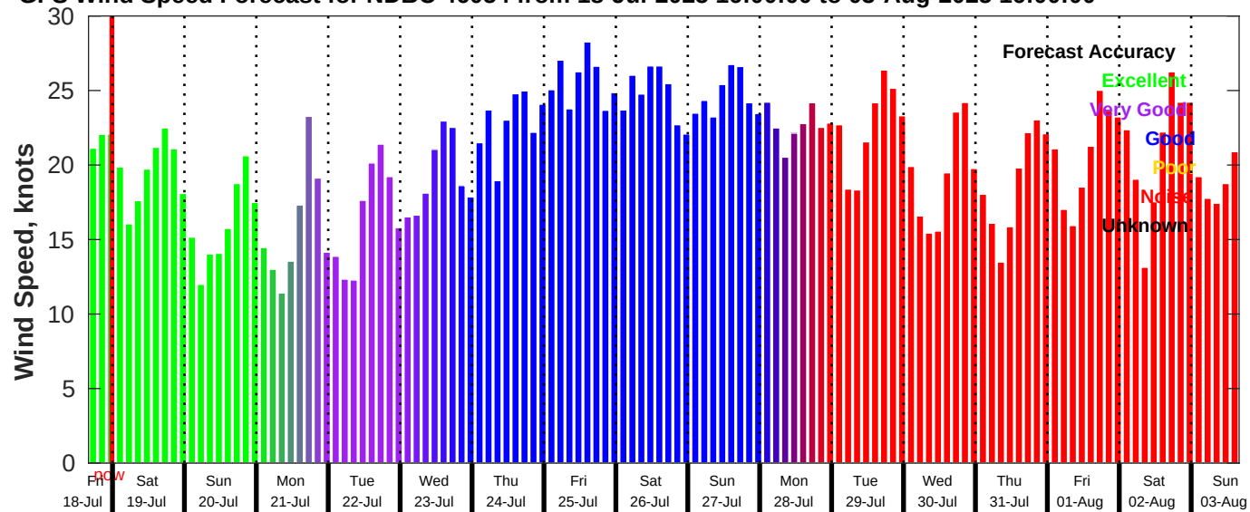
GFS Wind Speed Forecast for NDBC 46054 from 18-Jul-2025 16:00:00 to 03-Aug-2025 16:00:00
