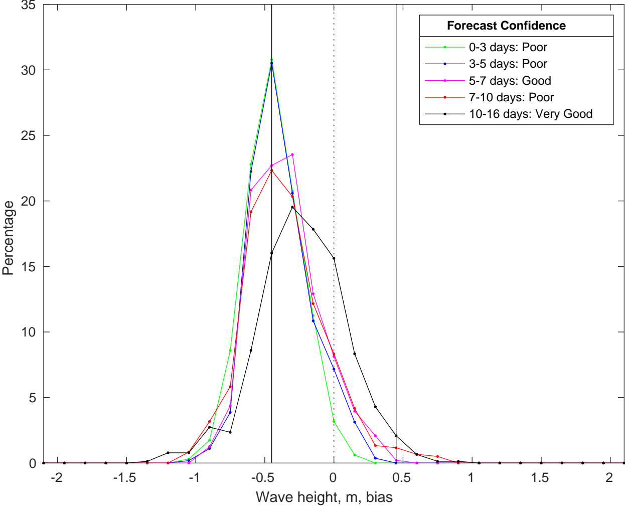
NDBC 46069 vs GFS Waves Bias Histogram: 19-Jul-2025
