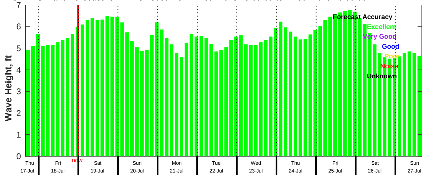
CMEMS Wave Forecast for NDBC 46069 from 17-Jul-2025 16:00:00 to 27-Jul-2025 16:00:00
