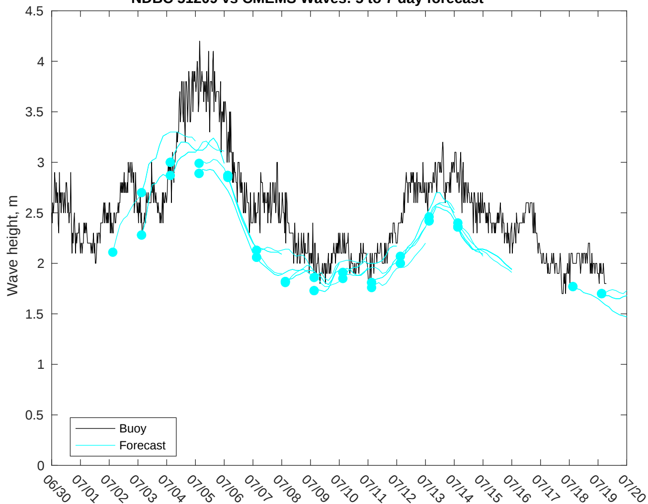
NDBC 51209 vs CMEMS Waves: 5 to 7 day forecast
