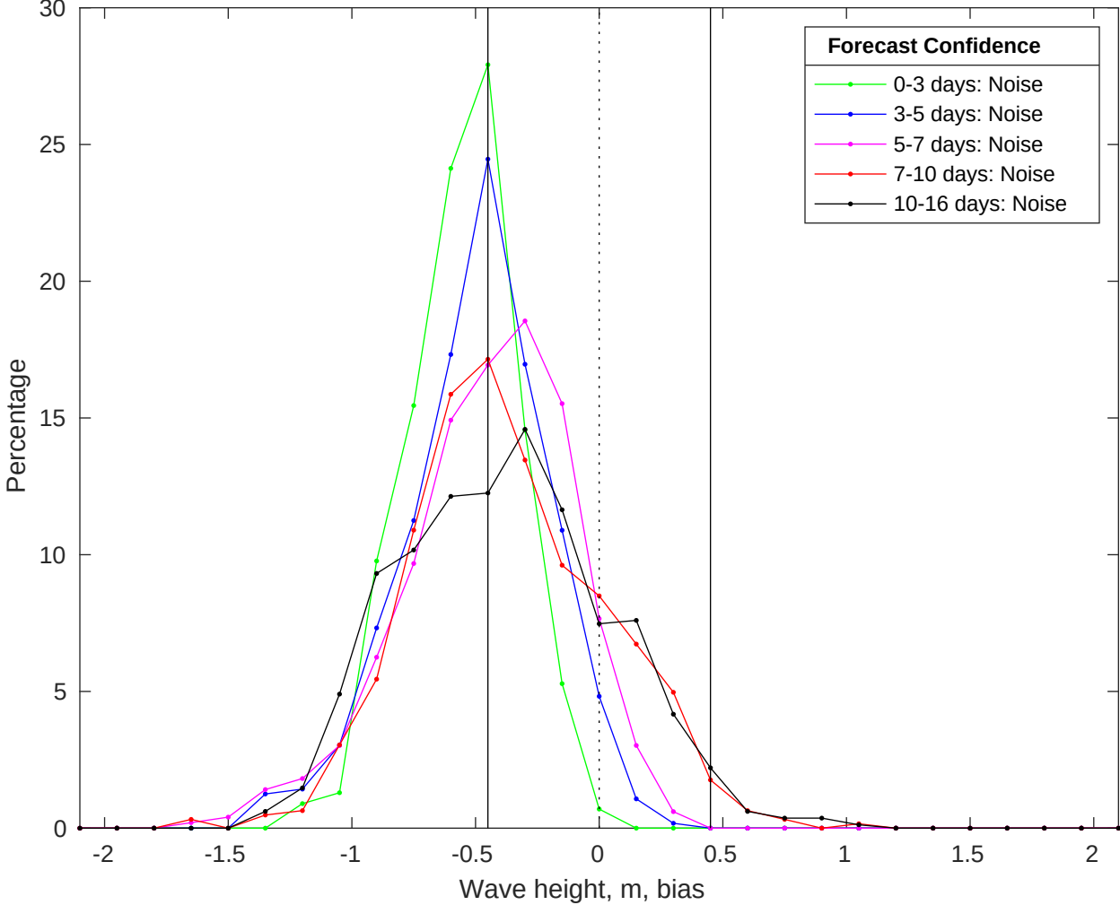
NDBC 51209 vs GFS Waves Bias Histogram: 19-Jul-2025
