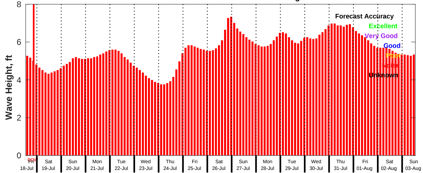
GFS Wave Forecast for NDBC 51209 from 18-Jul-2025 13:00:00 to 03-Aug-2025 13:00:00
