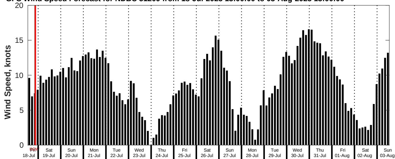
GFS Wind Speed Forecast for NDBC 51209 from 18-Jul-2025 13:00:00 to 03-Aug-2025 13:00:00
