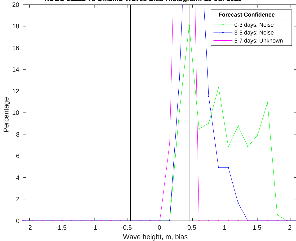
NDBC 51211 vs CMEMS Waves Bias Histogram: 19-Jul-2025
