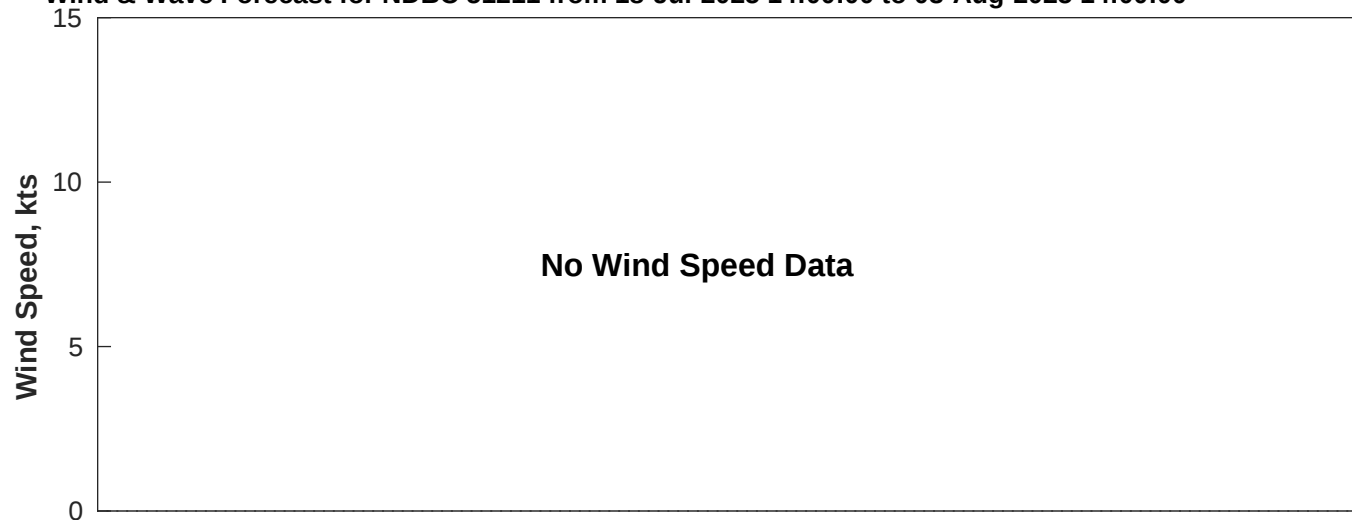
Wind & Wave Forecast for NDBC 51211 from 18-Jul-2025 14:00:00 to 03-Aug-2025 14:00:00
