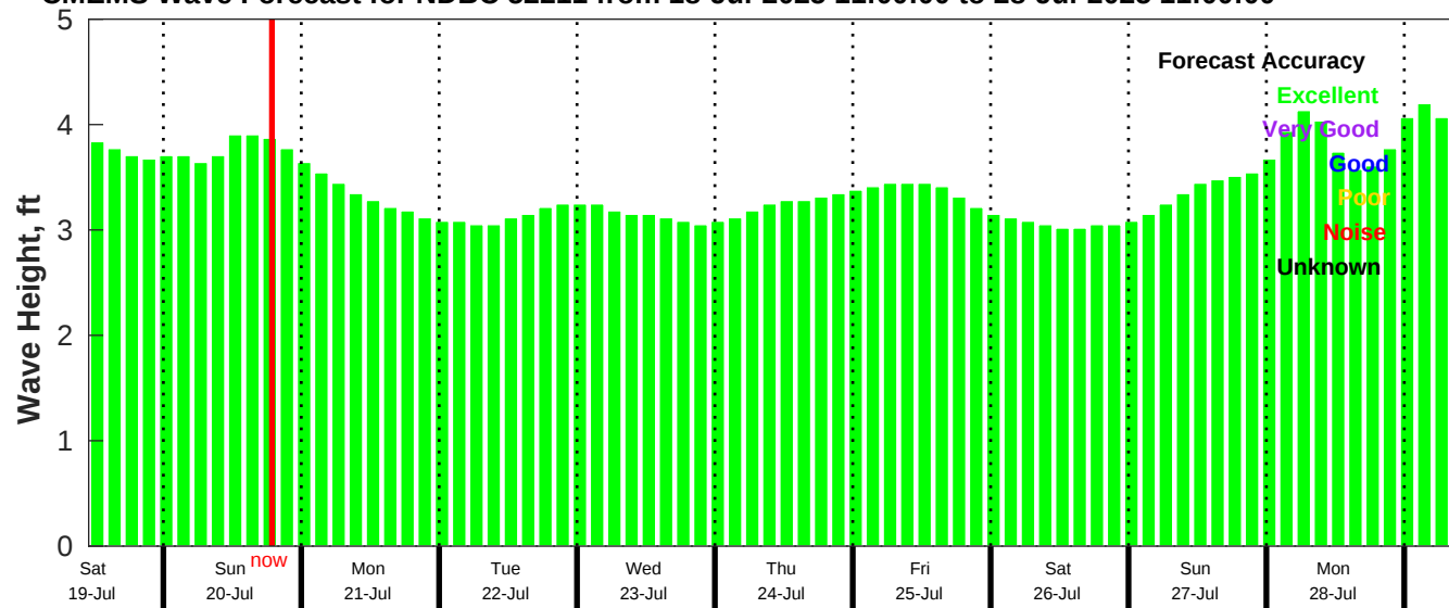
CMEMS Wave Forecast for NDBC 52211 from 18-Jul-2025 11:00:00 to 28-Jul-2025 11:00:00
