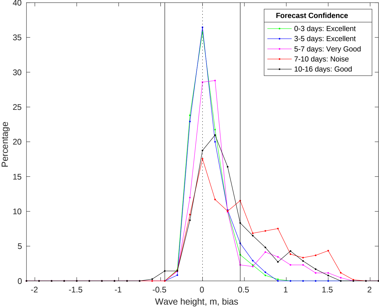
NDBC 52212 vs GFS Waves Bias Histogram: 19-Jul-2025
