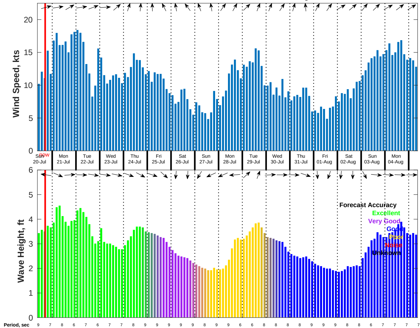
Wind & Wave Forecast for NDBC 52212 from 19-Jul-2025 09:00:00 to 04-Aug-2025 09:00:00
