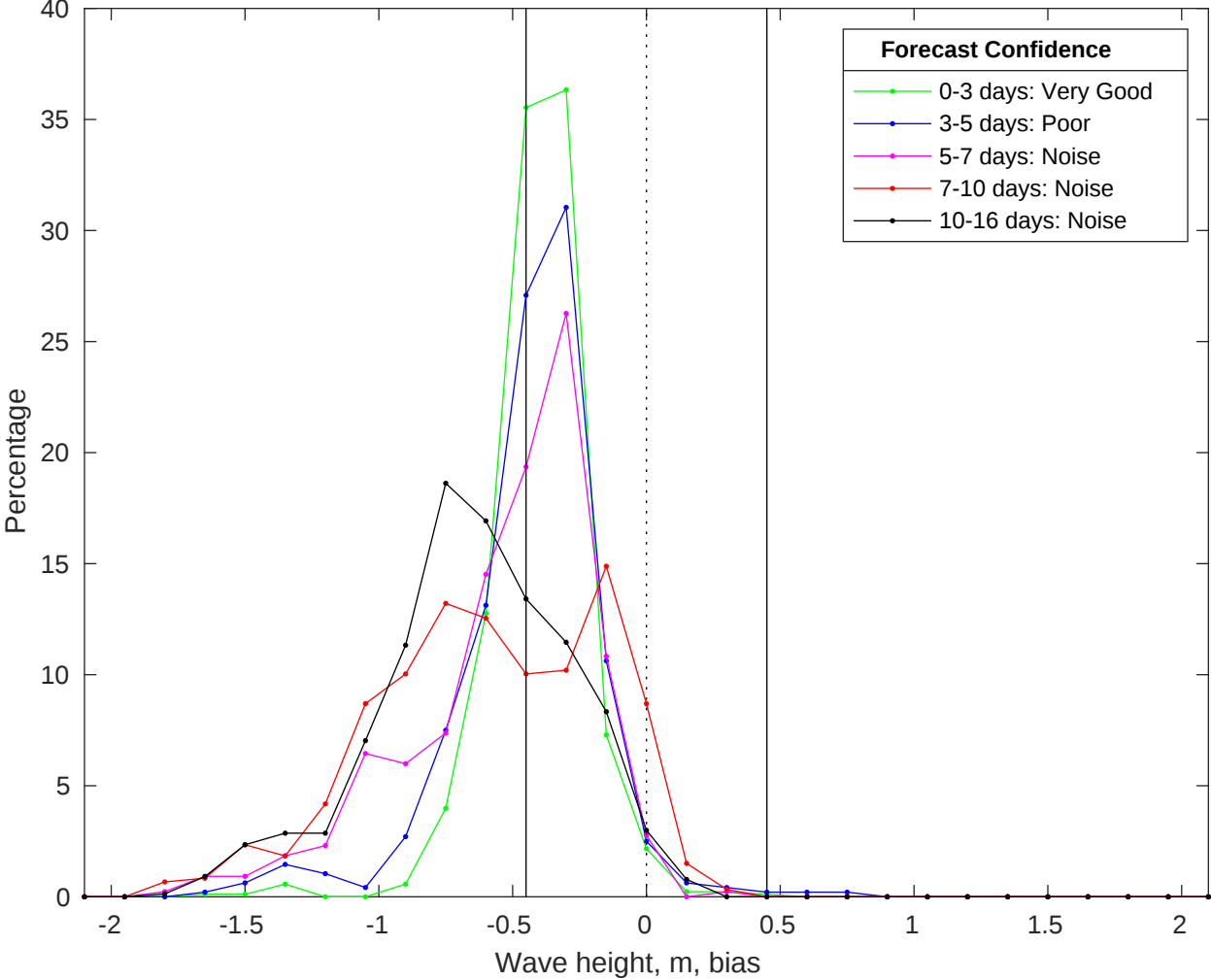
NDBC 52213 vs GFS Waves Bias Histogram: 19-Jul-2025
