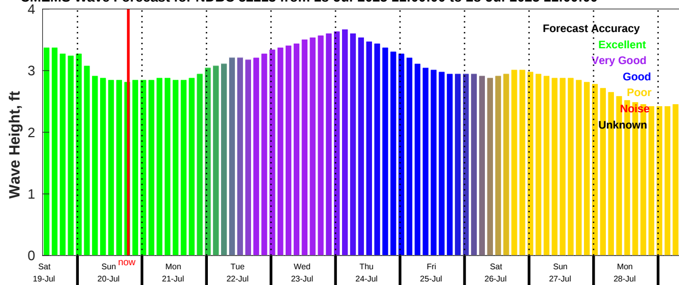
CMEMS Wave Forecast for NDBC 52213 from 18-Jul-2025 11:00:00 to 28-Jul-2025 11:00:00
