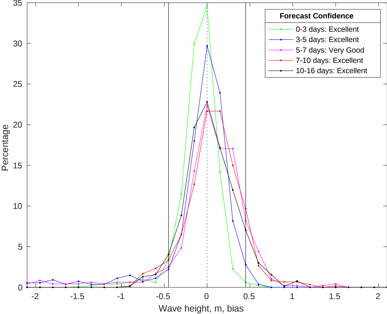
NDBC 41004 vs GFS Waves Bias Histogram: 20-Jul-2025
