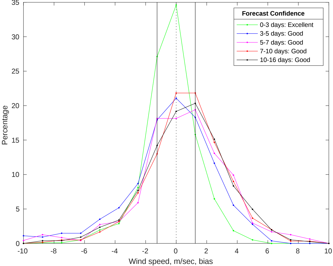
NDBC 41004 vs GFS Winds Bias Histogram: 20-Jul-2025
