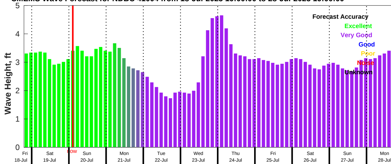
CMEMS Wave Forecast for NDBC 41004 from 18-Jul-2025 19:00:00 to 28-Jul-2025 19:00:00
