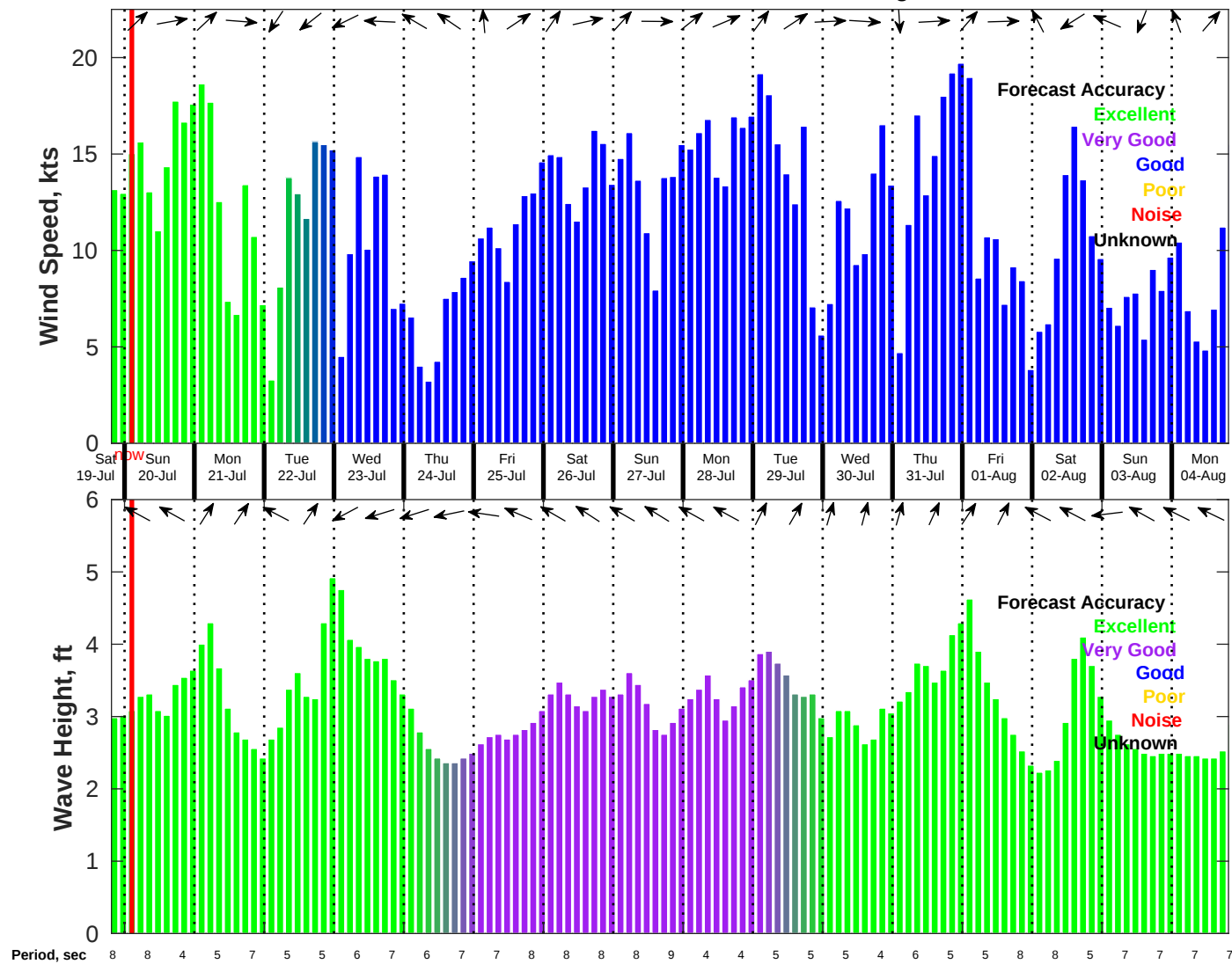
Wind & Wave Forecast for NDBC 41004 from 19-Jul-2025 19:00:00 to 04-Aug-2025 19:00:00
