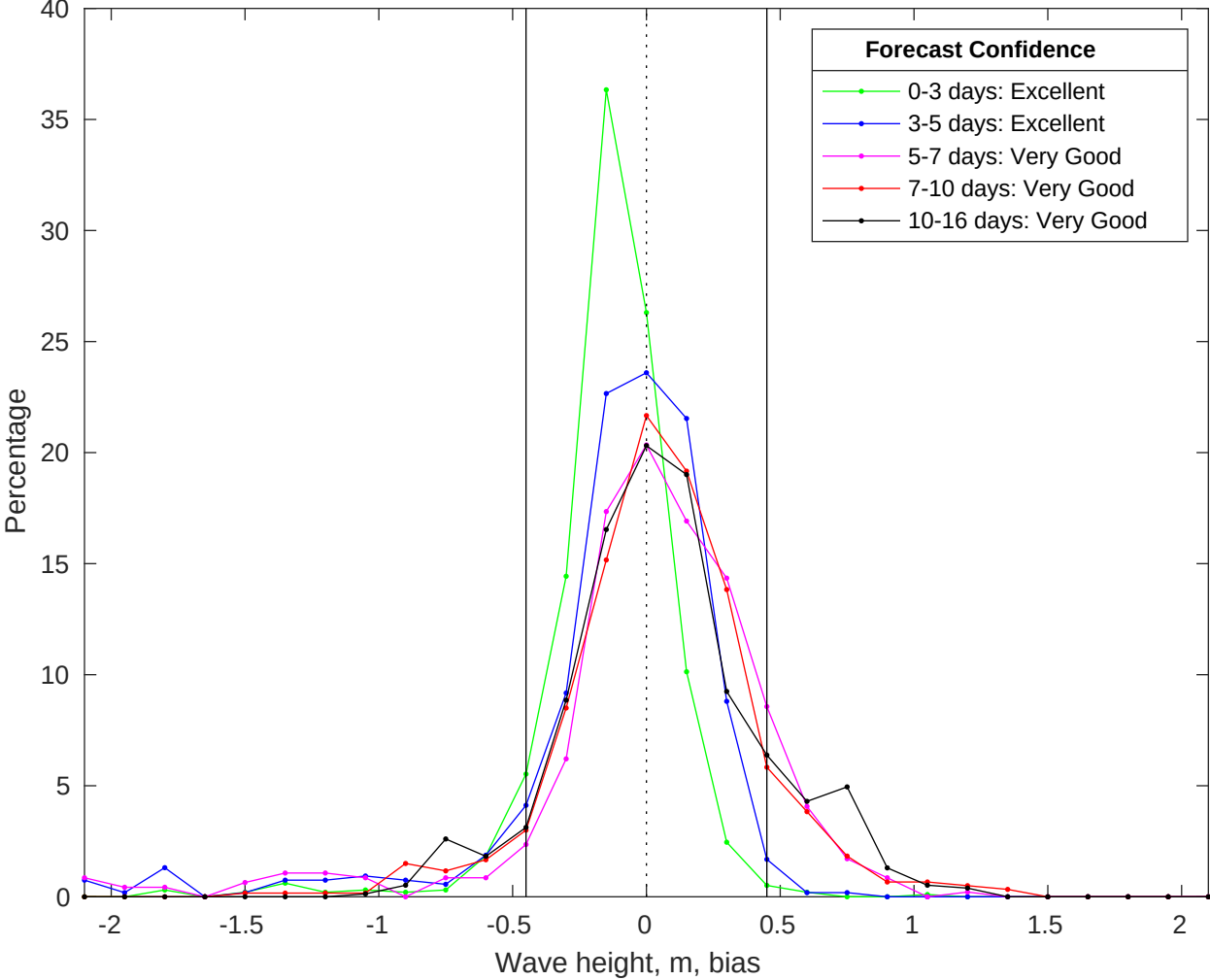
NDBC 41013 vs GFS Waves Bias Histogram: 20-Jul-2025
