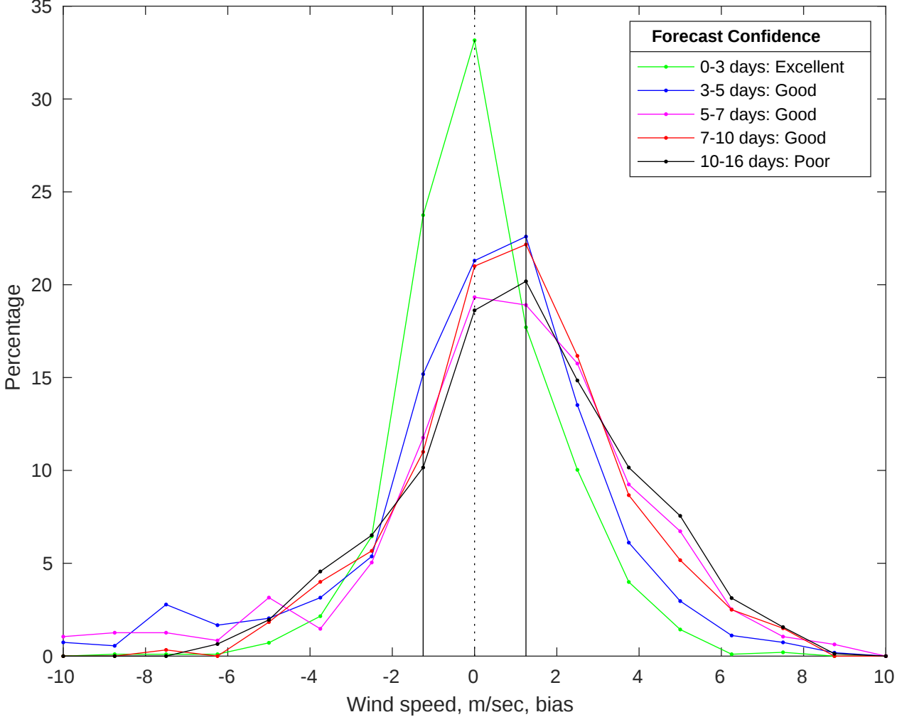
NDBC 41013 vs GFS Winds Bias Histogram: 20-Jul-2025
