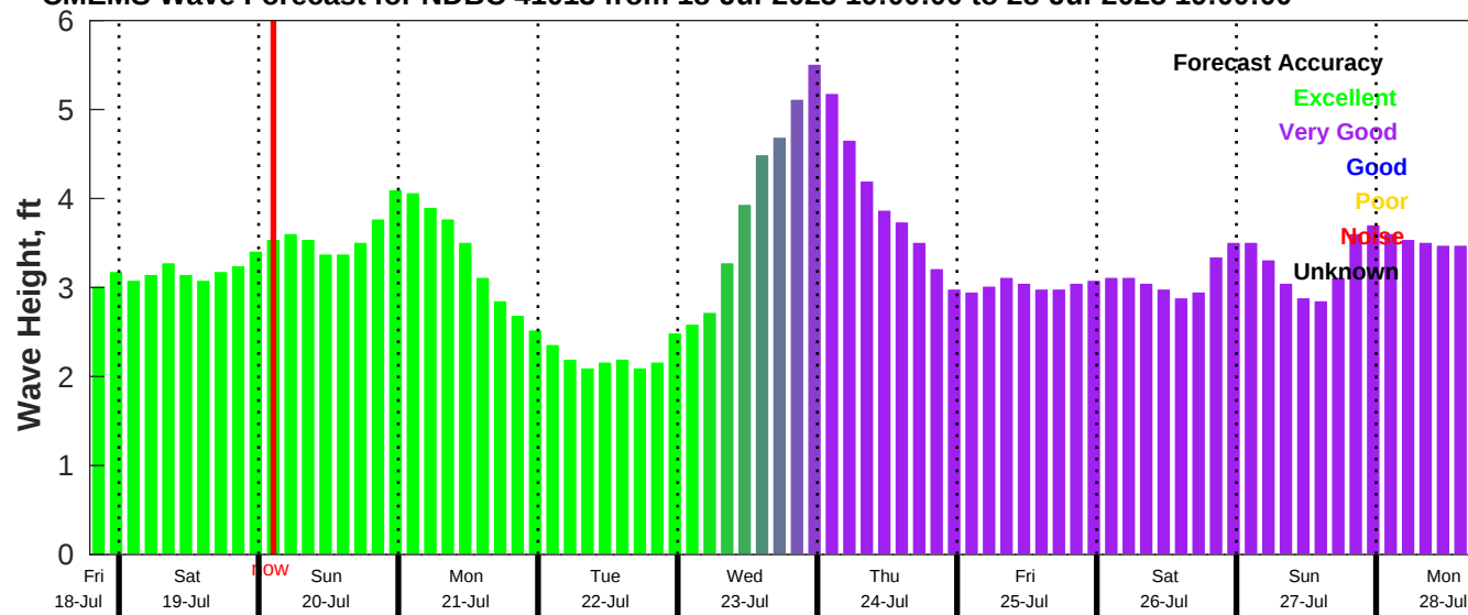
CMEMS Wave Forecast for NDBC 41013 from 18-Jul-2025 19:00:00 to 28-Jul-2025 19:00:00
