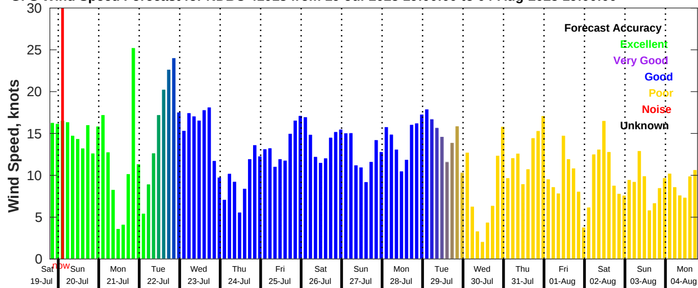
GFS Wind Speed Forecast for NDBC 41013 from 19-Jul-2025 19:00:00 to 04-Aug-2025 19:00:00
