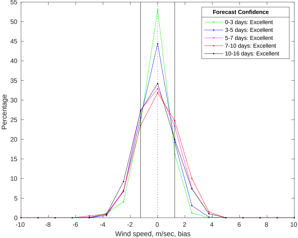
NDBC 41040 vs GFS Winds Bias Histogram: 20-Jul-2025
