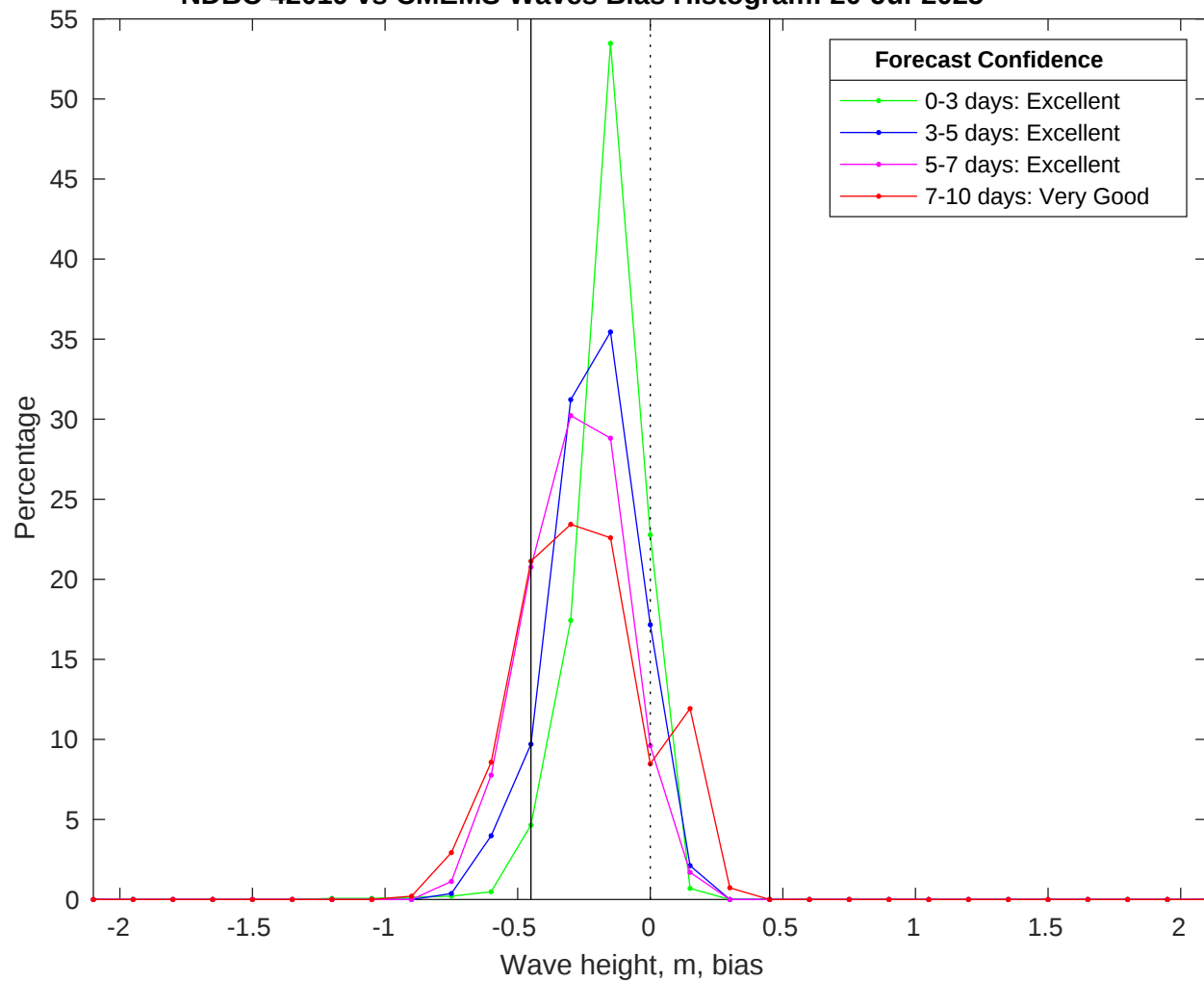
NDBC 42019 vs CMEMS Waves Bias Histogram: 20-Jul-2025
