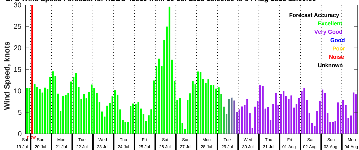
GFS Wind Speed Forecast for NDBC 42019 from 19-Jul-2025 18:00:00 to 04-Aug-2025 18:00:00
