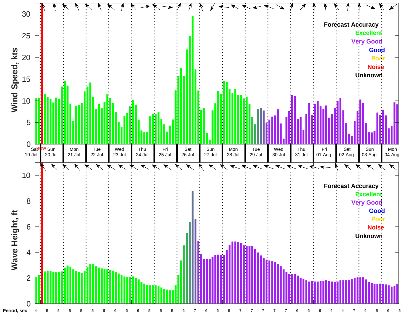
Wind & Wave Forecast for NDBC 42019 from 19-Jul-2025 18:00:00 to 04-Aug-2025 18:00:00
