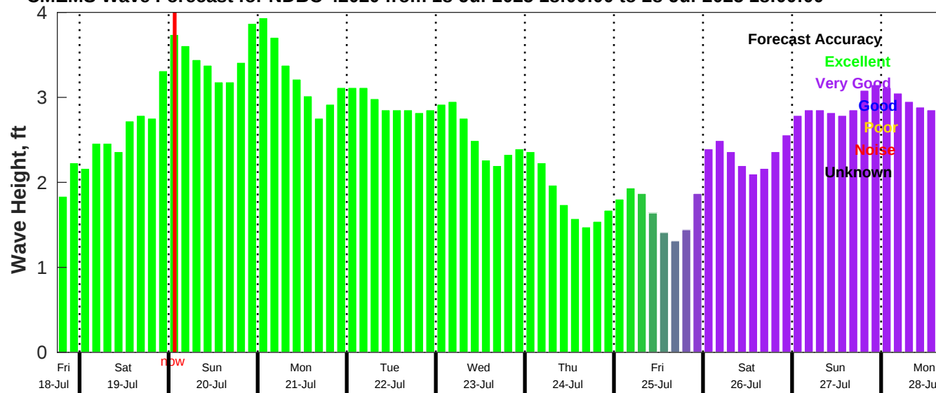
CMEMS Wave Forecast for NDBC 42020 from 18-Jul-2025 18:00:00 to 28-Jul-2025 18:00:00
