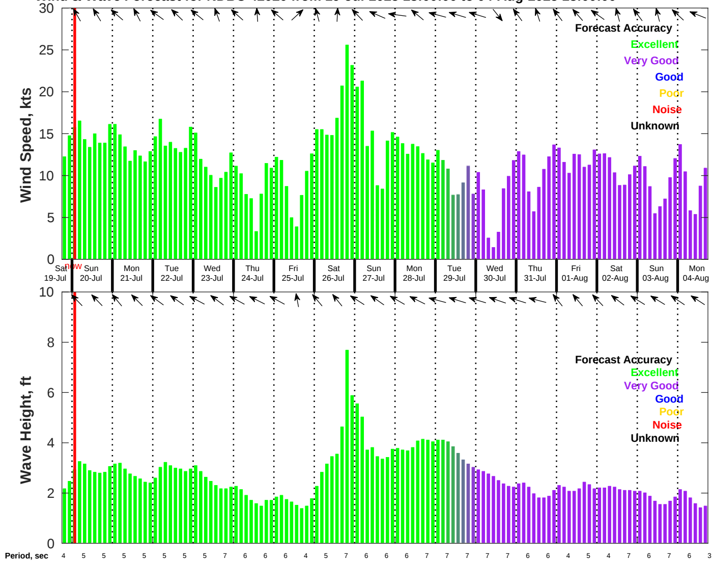
Wind & Wave Forecast for NDBC 42020 from 19-Jul-2025 18:00:00 to 04-Aug-2025 18:00:00
