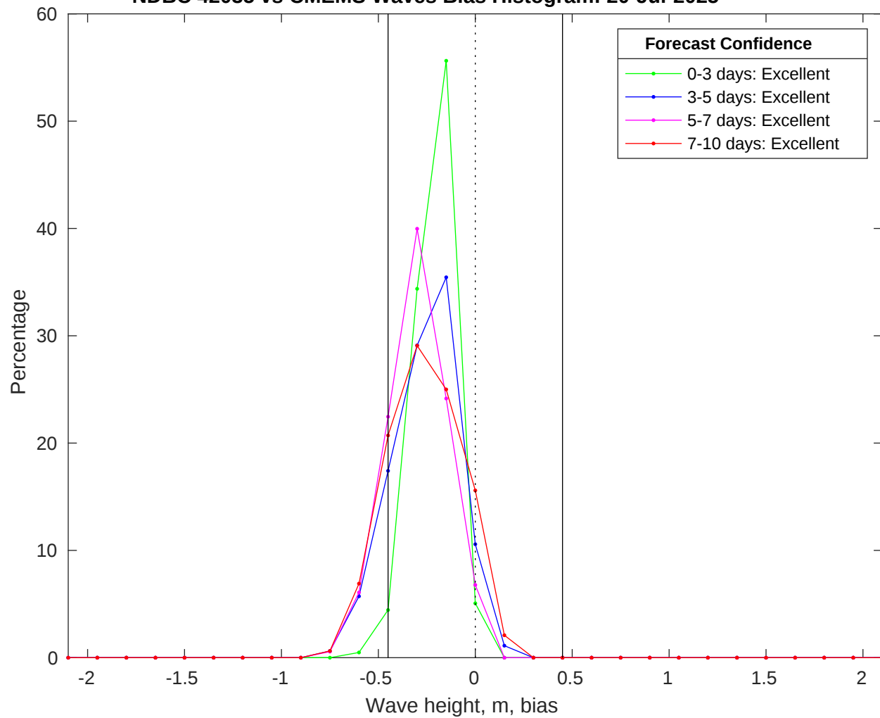
NDBC 42035 vs CMEMS Waves Bias Histogram: 20-Jul-2025
