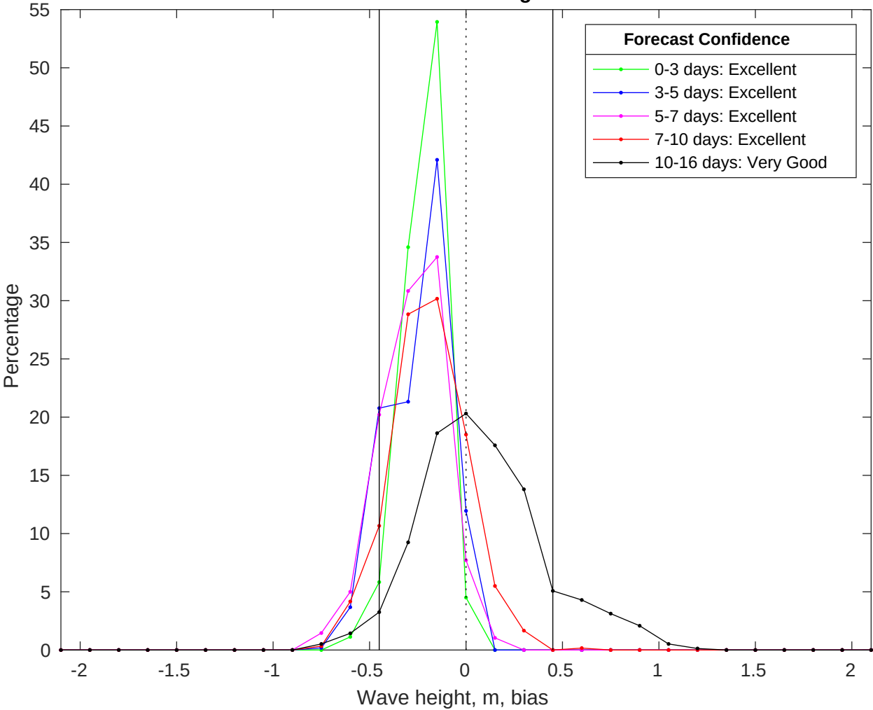
NDBC 42035 vs GFS Waves Bias Histogram: 20-Jul-2025
