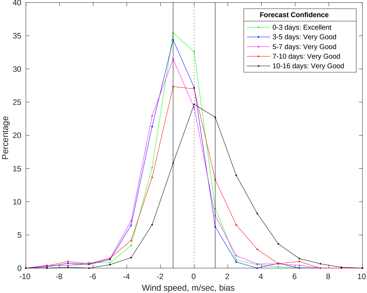
NDBC 42035 vs GFS Winds Bias Histogram: 20-Jul-2025
